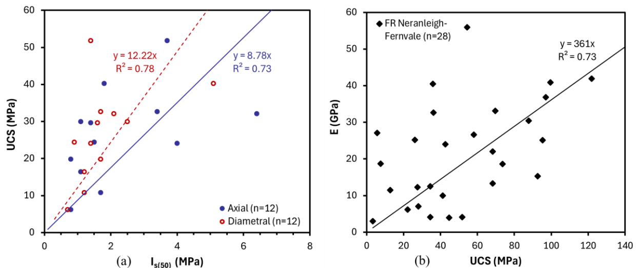
Figure 20. City / South Bank (a) UCS to I_{s(50)} correlations and (b) correlation between modulus and UCS for Fresh Neranleigh–Fernvale beds (Look and Griffiths 2001)
