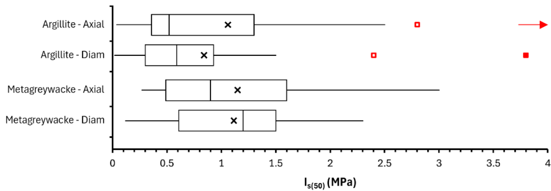
Figure 13. Centenary Bridge variation of I_{s(50)} results with rock material type and test direction
