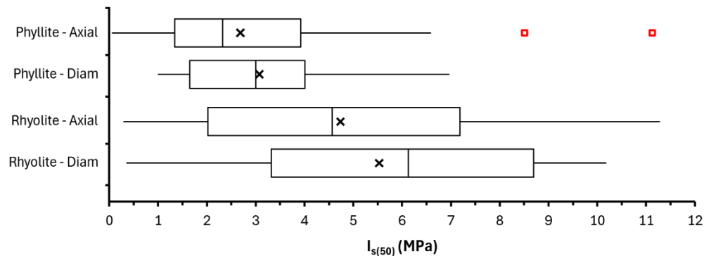
Figure 16. Indooroopilly variation of I_{s(50)} results with rock material type and test direction
