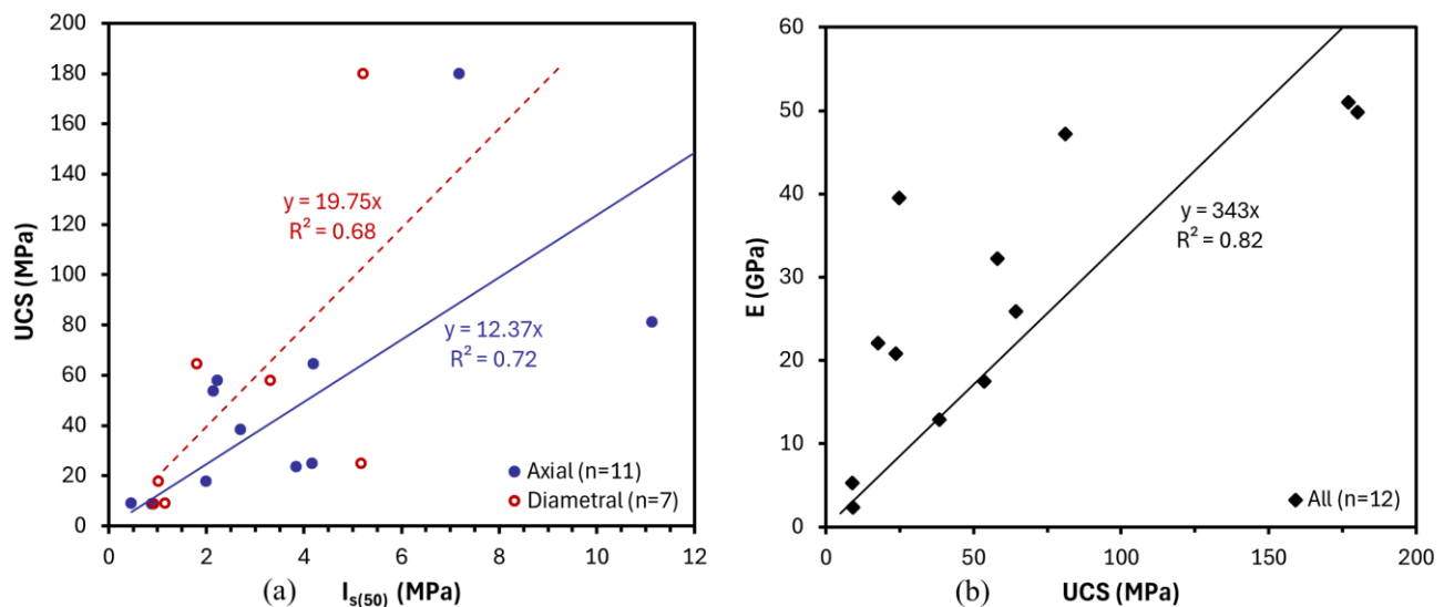
Figure 17. Indooroopilly (a) UCS to I_{s(50)} correlations and (b) correlation between modulus and UCS
