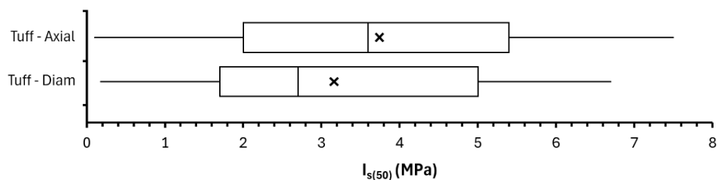
Figure 22. City / New Farm tuff variation of I_{s(50)} results with test direction
