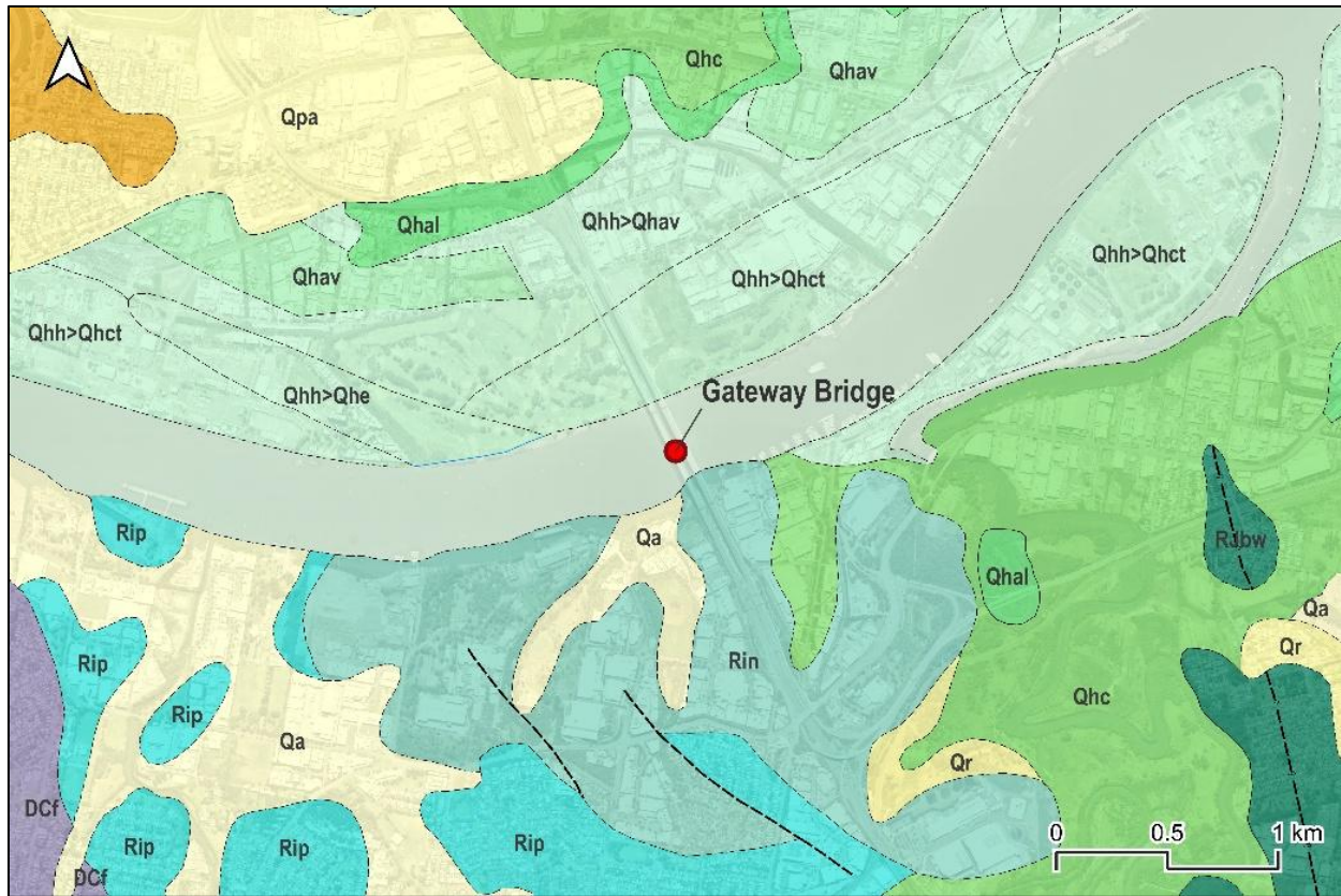
Figure 24. Gateway Bridge surface geology (Geological Survey of Queensland 2023)
