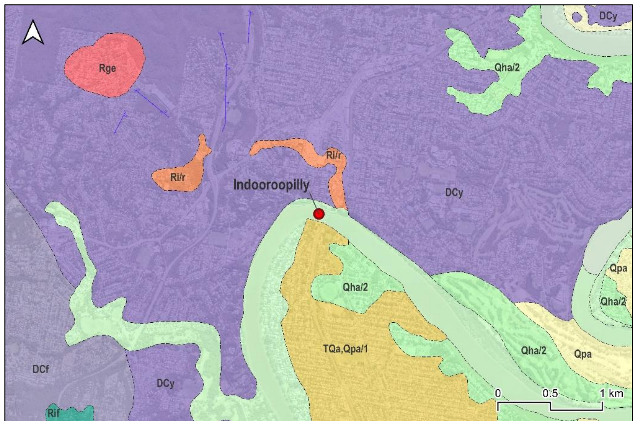
Figure 15. Indooroopilly surface geology (Geological Survey of Queensland 2023)
