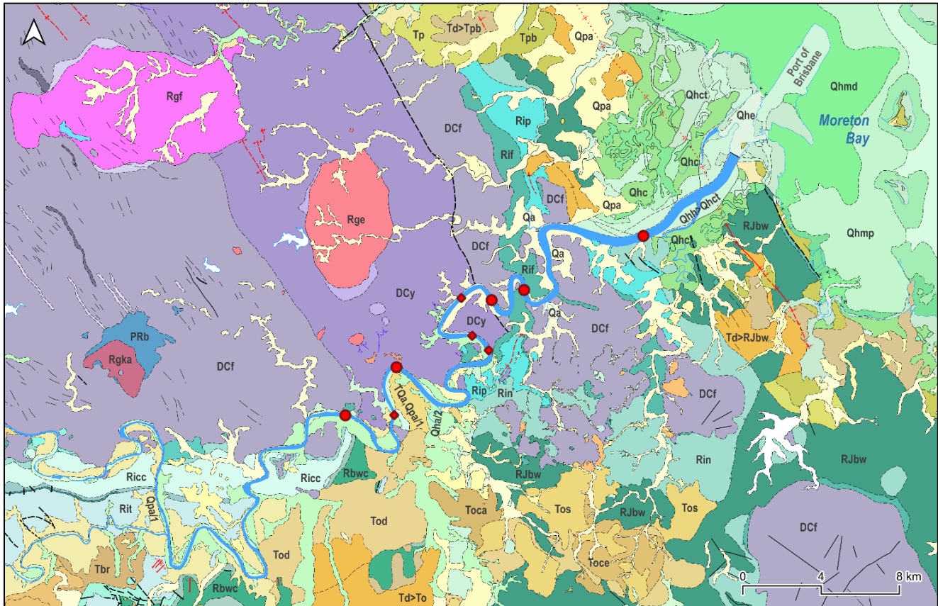
Figure 3. Surface geology of the Brisbane River study area (Geological Survey of Queensland 2023)
