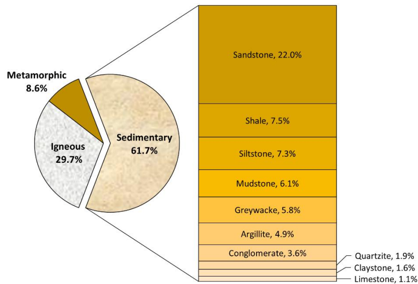
Figure 9. Common lithologies for infrastructure related sites across Queensland
