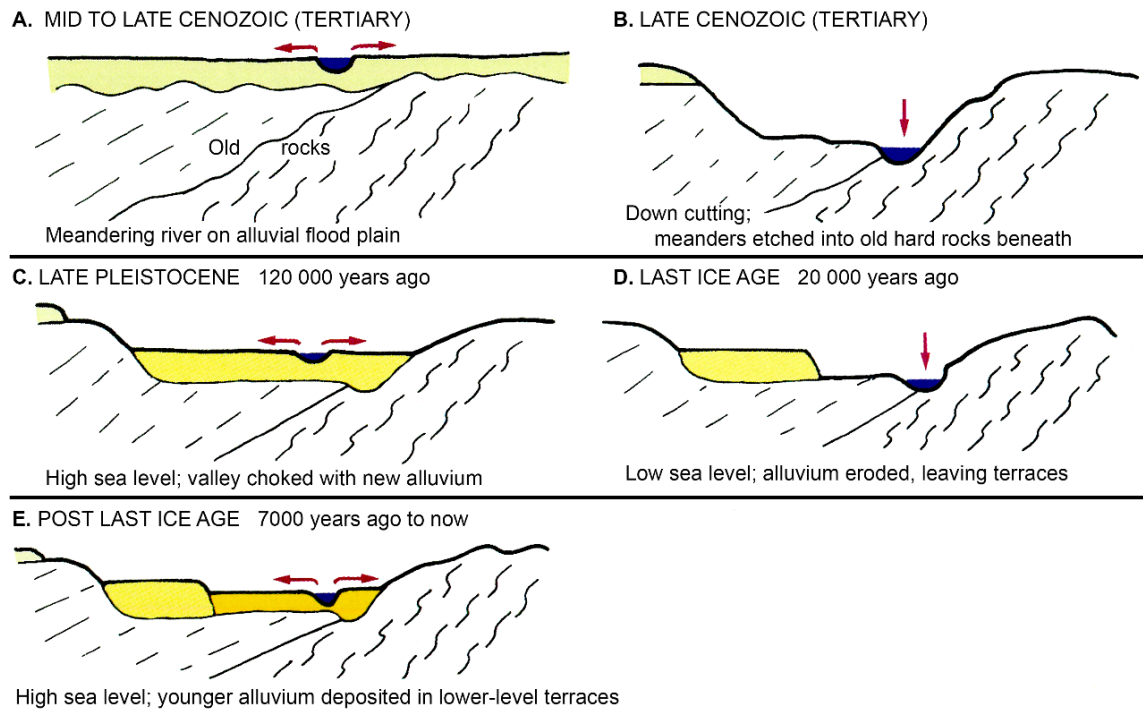
Figure 4. Progressive development of the Brisbane River valley (Willmott, 2012)
