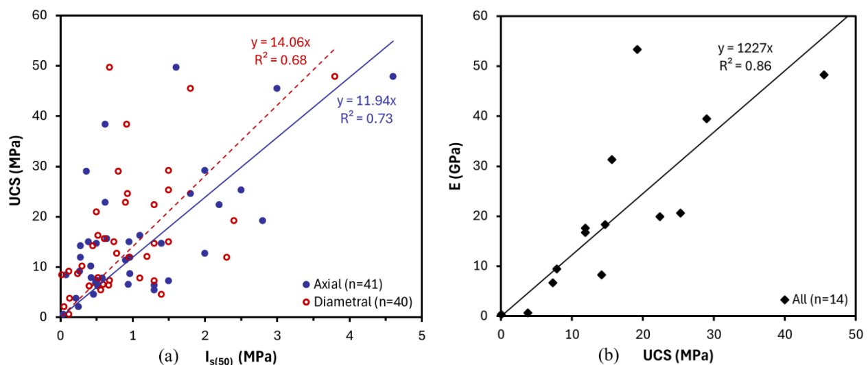
Figure 14. Centenary Bridge (a) UCS to I_{s(50)} correlations and (b) E to UCS correlation
