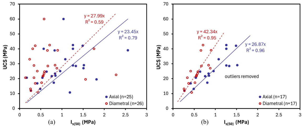
Figure 26. Gateway Bridge sandstone–siltstone UCS to I_{s(50)} correlations (a) with outliers, (b) without outliers (Look and Wijeyakulasuriya 2009)
