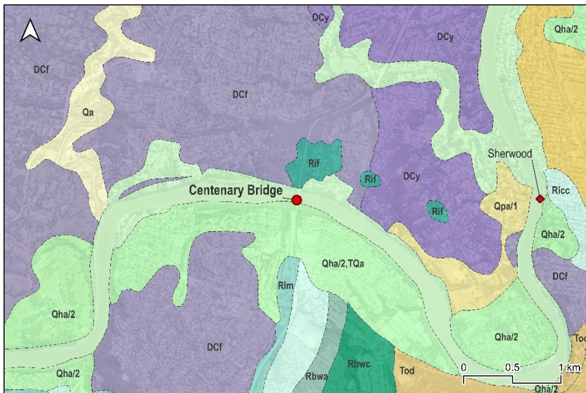
Figure 12. Centenary Bridge surface geology (Geological Survey of Queensland 2023)
