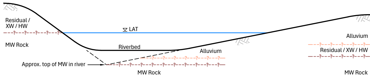
Figure 5. Conceptual upstream geometry (facing Moreton Bay)
