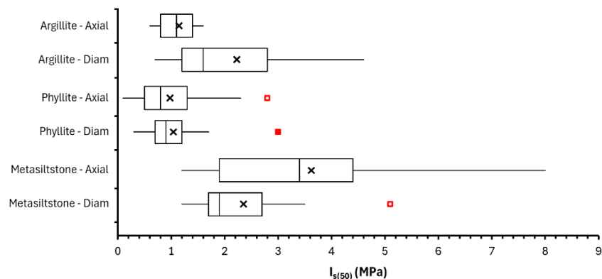
Figure 19. City / South Bank variation of I_{s(50)} results with rock material type and test direction
