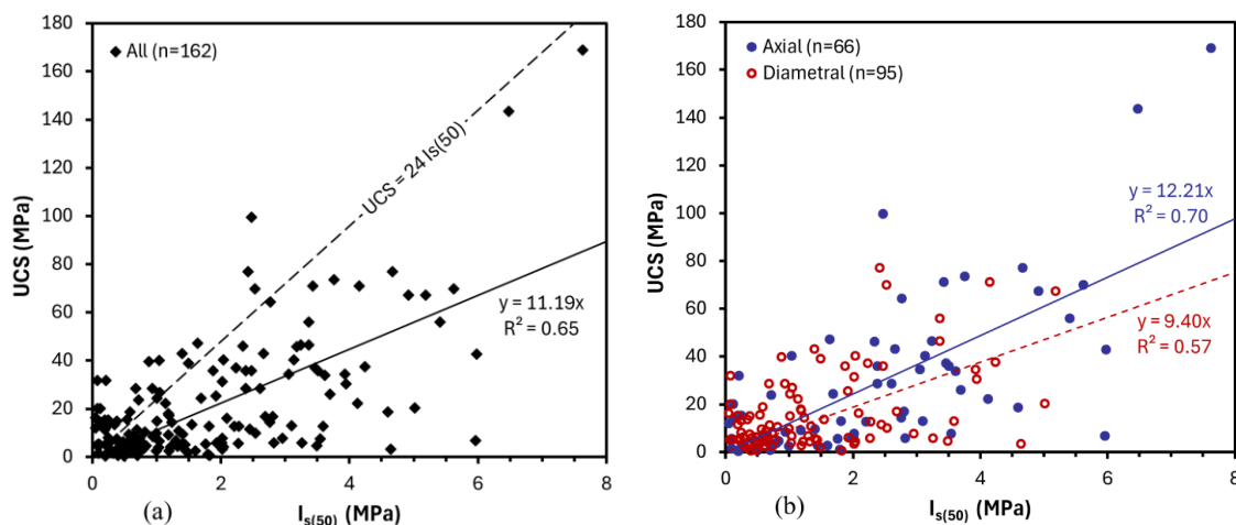
Figure 10. Brisbane rock strength: (a) UCS to I_{s(50)} correlation; (b) showing effect of anisotropy (Look and Griffiths 2001, 2004)
