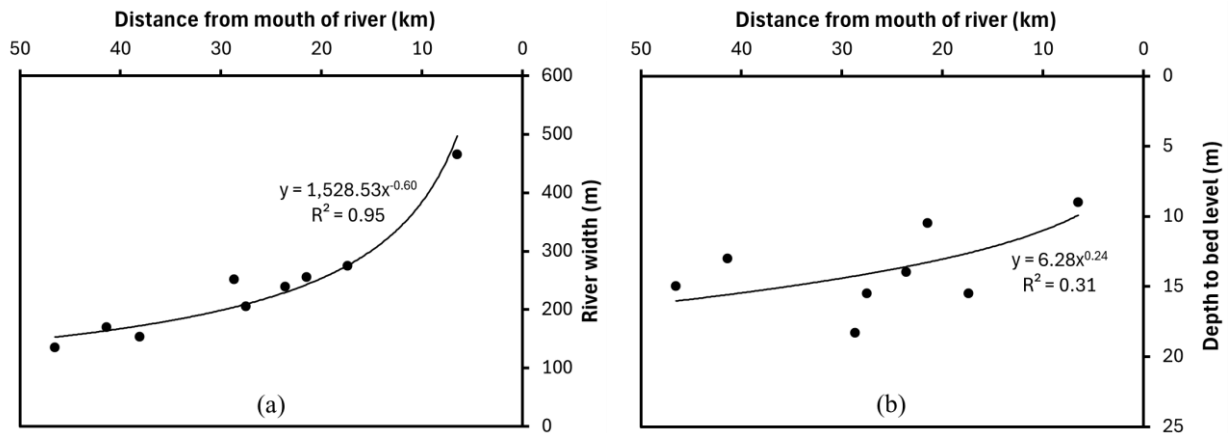
Figure 7. Variation of (a) river width and (b) depth to riverbed level with distance from mouth of river
