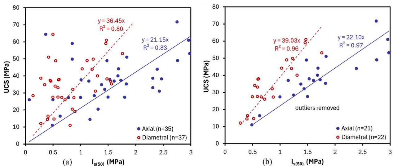
Figure 27. Gateway Bridge sandstone–mudstone UCS to I_{s(50)} correlations (a) with outliers, (b) without outliers (Look and Wijeyakulasuriya 2009)
