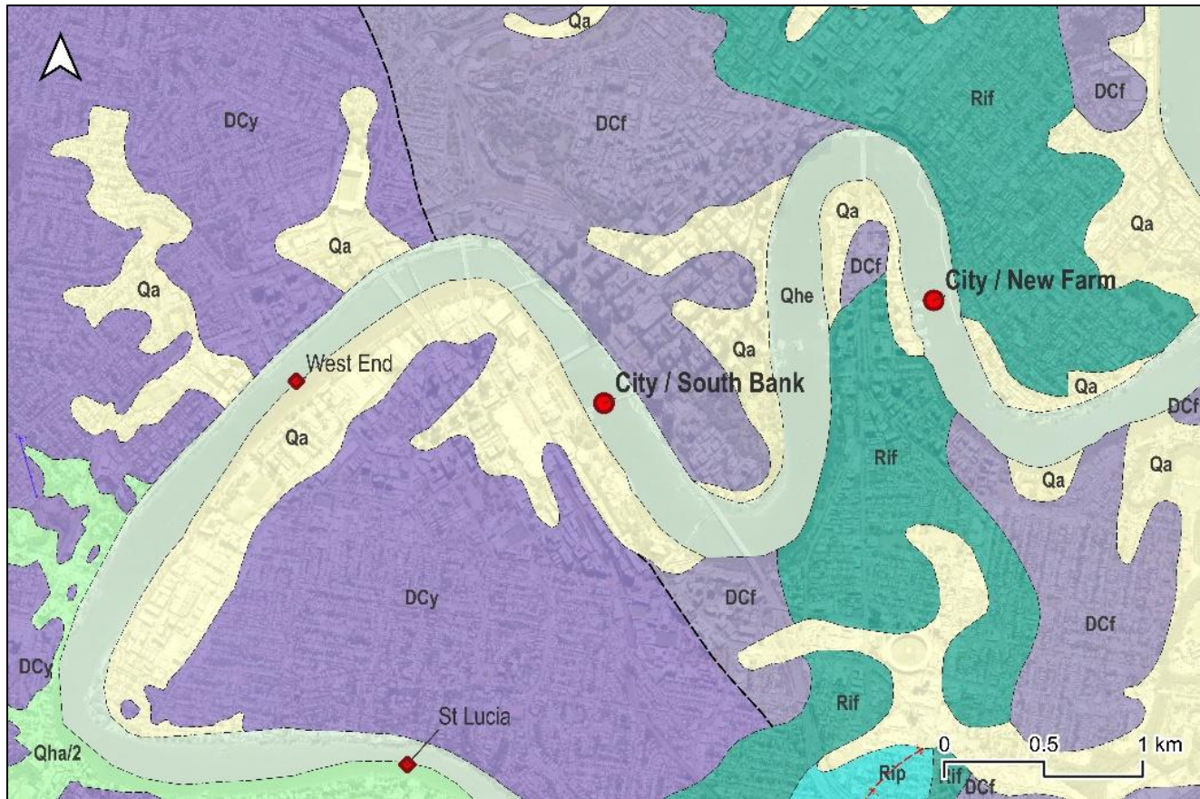
Figure 18. City / South Bank surface geology (Geological Survey of Queensland 2023)
