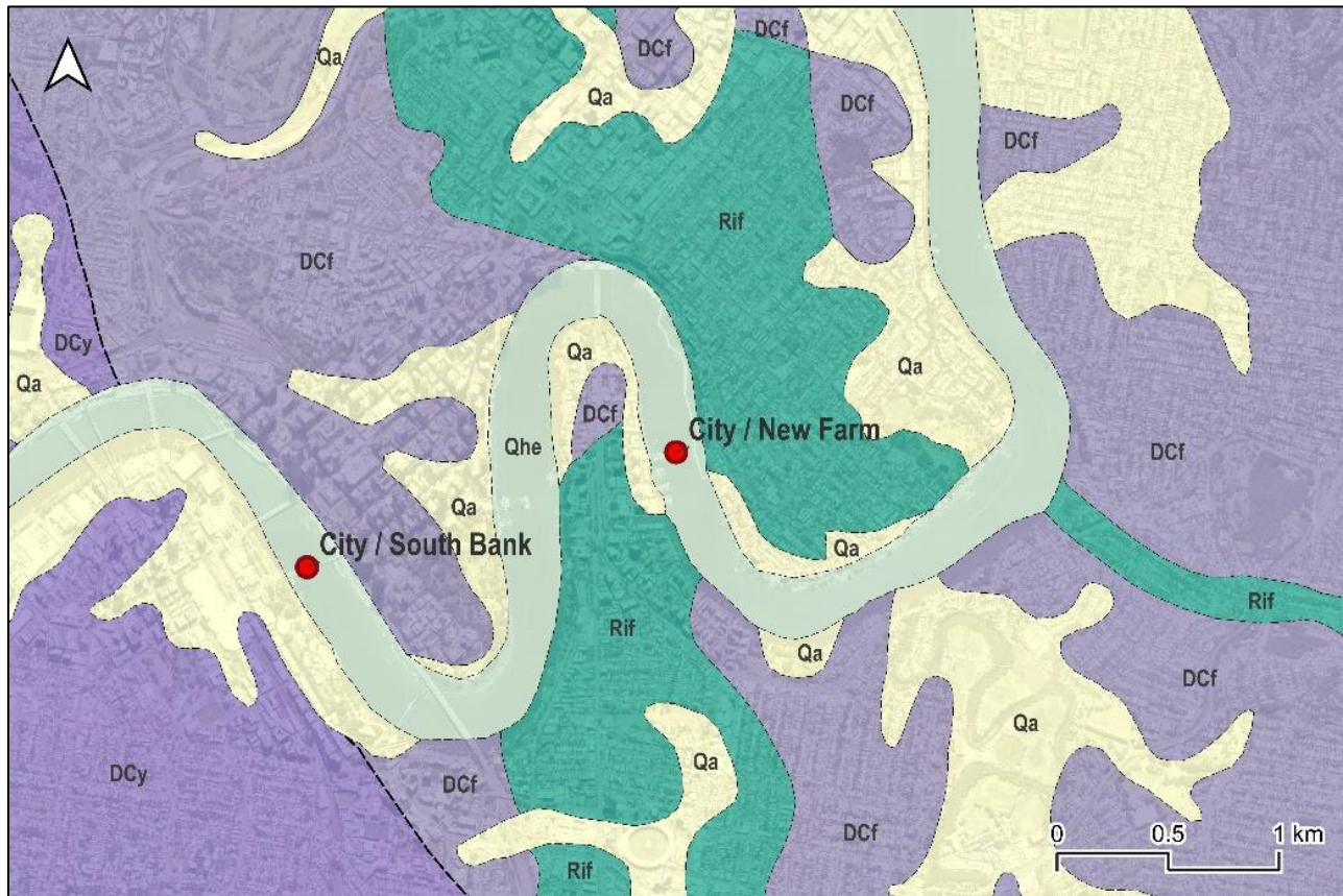
Figure 21. City / New Farm surface geology (Geological Survey of Queensland 2023)
