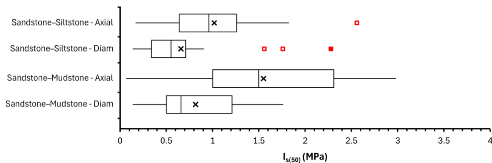
Figure 25. Gateway Bridge variation of I_{s(50)} results with rock material type and test direction
