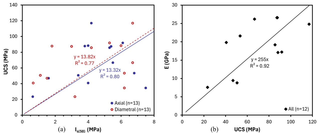
Figure 23. City / New Farm tuff (a) UCS to I_{s(50)} correlations and (b) correlation between modulus and UCS
