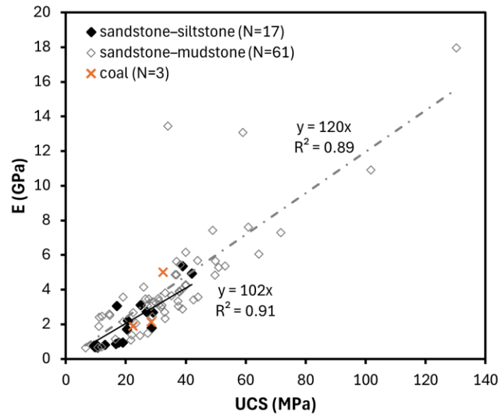
Figure 28. Gateway Bridge correlation between modulus and UCS
