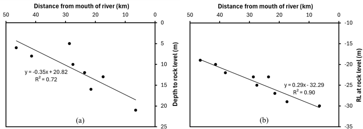
Figure 8. Variation of (a) depth to rock level and (b) RL at rock level with distance from mouth of river
