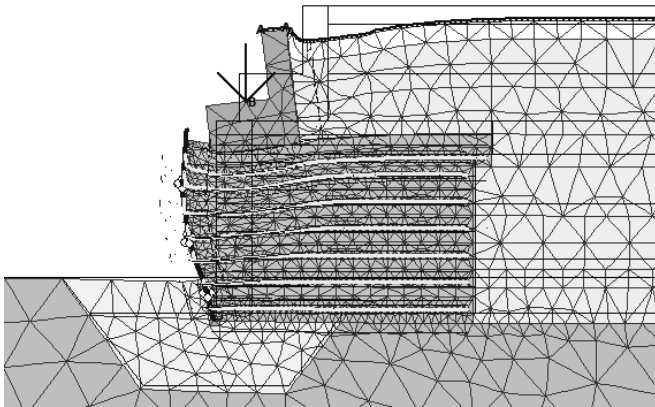
Figure 14. Deformed mesh (a) and shear strains (b) at post-construction serviceability stages. Base case.
