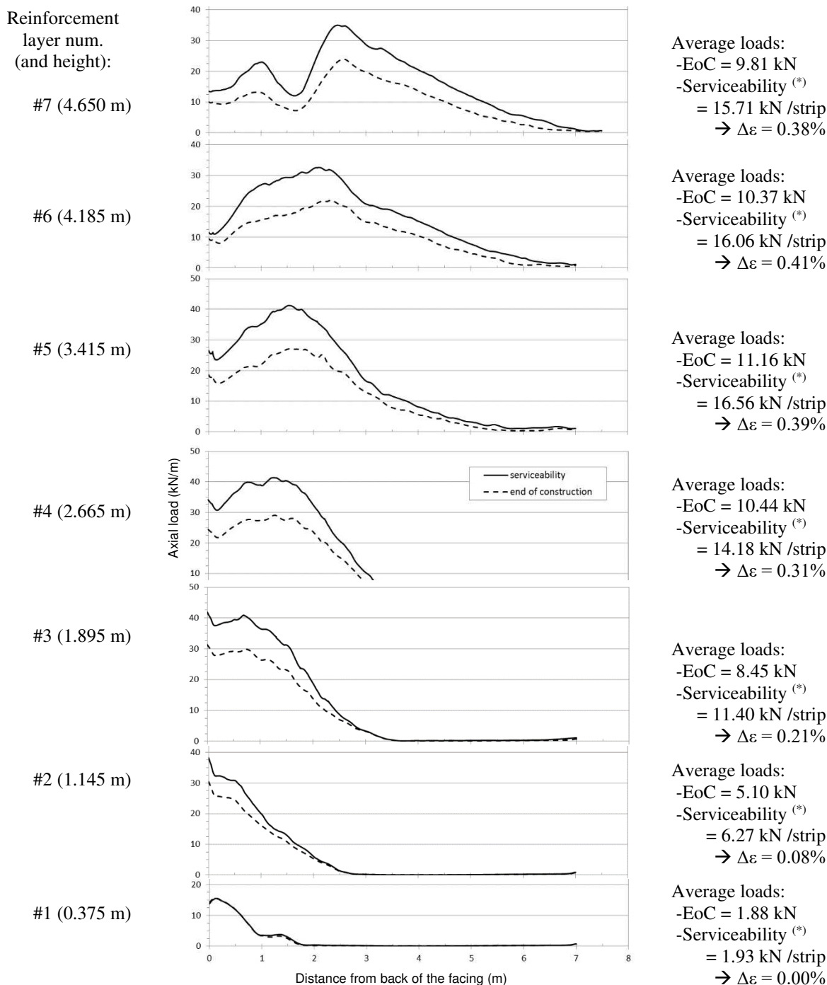
Figure 15. Reinforcement axial load (kN/m) distribution at the end of construction and under serviceability long-term scenario (*) 100% of the LL's application). Base case.
