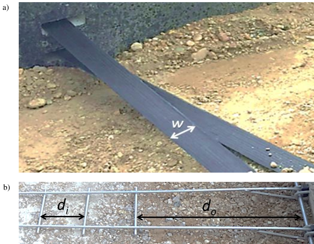
Figure 2. Details of the VSOL ® wall reinforcement types used in the D4R7 Project: (a) polymeric strips and (b) galvanized steel ladders and related connection systems (void formed and clevis loops, respectively).
