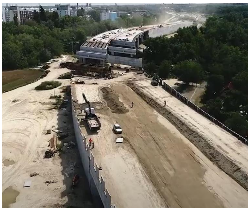
Figure 4. Back-to-back D4R7 reinforced soil walls during construction.
