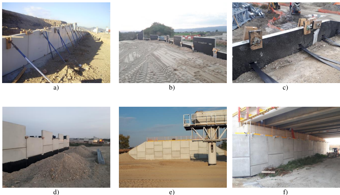
Figure 9. D4R7 Project VSoL ® reinforced soil bridge abutment construction stages: (a) 1 st panel row installation, (b) backfilling, (c) polymeric strips placement, (d) frontal embedment detail, (e) frontal view, and (f) bridge deck arrangement.
