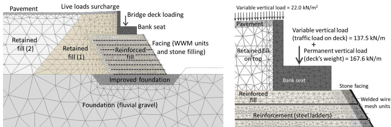
Figure 18. FEM 2D model mesh generated: (a) general model, and (b) bank seat with loading features detail.
