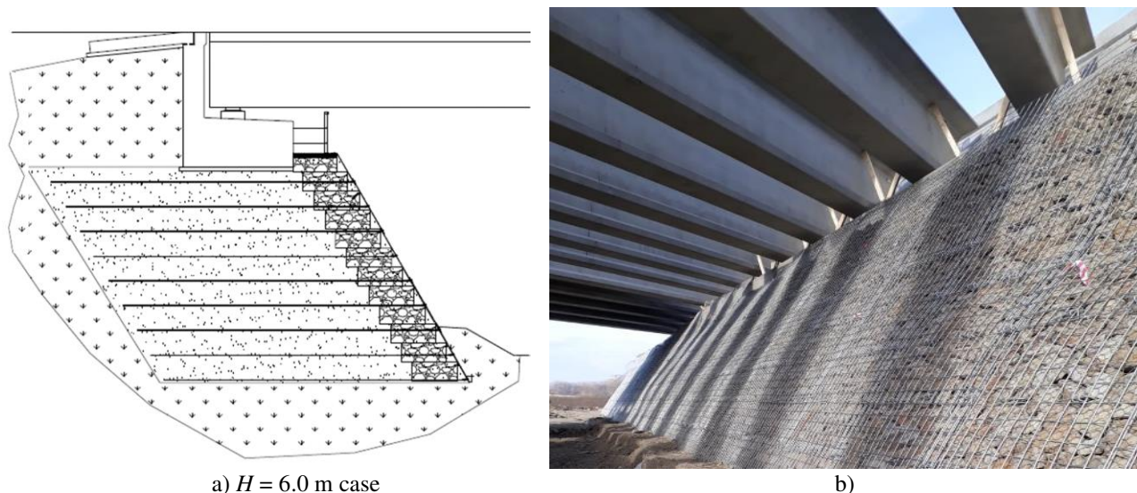
Figure 7. Bridge abutment reinforced soil slope type with WWM stone facing: (a) detailed section and (b) as-built (DAR7 Section 201-02).
