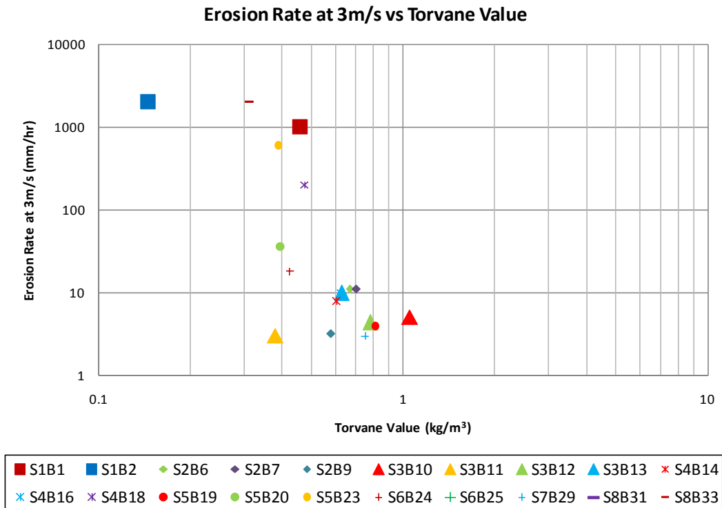
Figure 33. Erosion rate at 3m/s vs. Torvane values.
