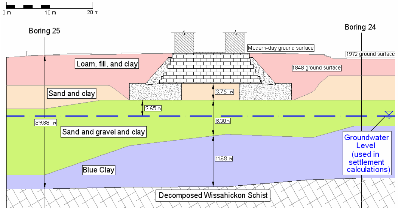
Figure 8. Generalized stratigraphy under the Washington Monument.
