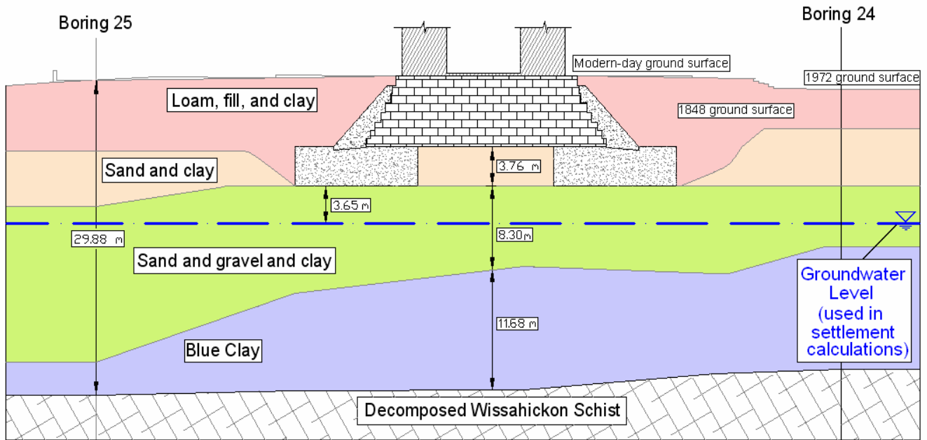
Figure 8. Generalized stratigraphy under the Washington Monument.
