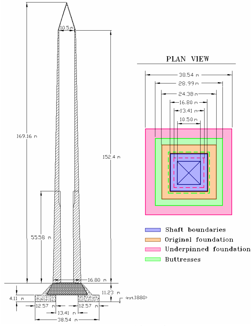
Figure 1. Dimensions of the Washington Monument.
