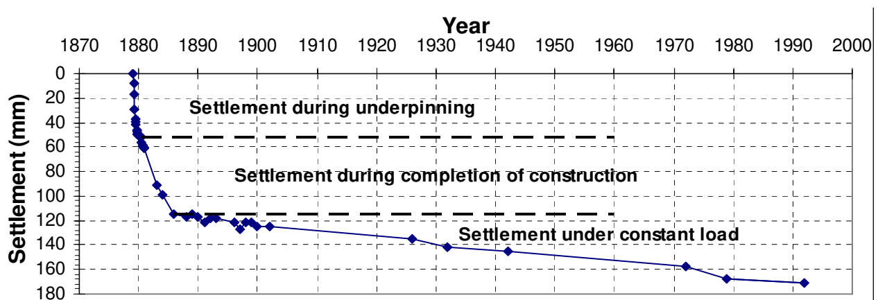
Figure 6. Settlement of the Washington Monument since underpinning (MRCE, 2002).
