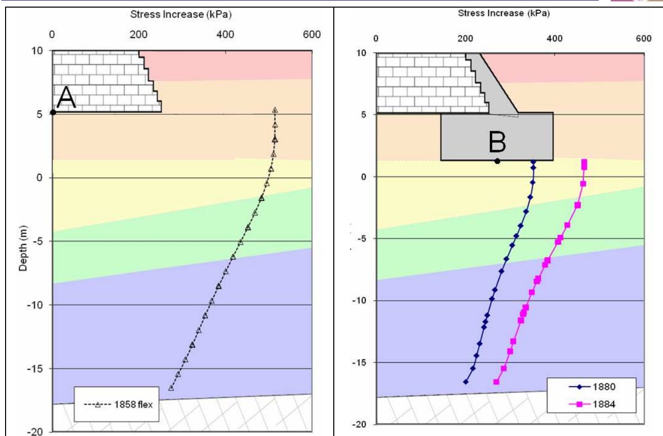
Figure 11. Increase in stress: A) below the center A of the 1858 foundation (flexible case), B) below the center B of the underpinning (flexible case).
